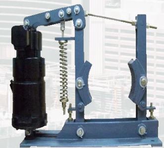
Thruster Brake Assembly 100-500 Dia.
